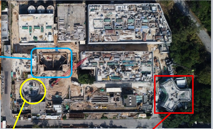
Excavation and lateral support works for Sludge Centrifuge House 污泥離心機大樓的挖掘與側向承托工程
